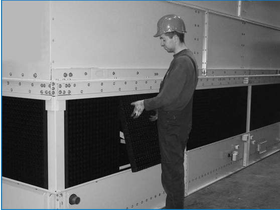
Remove combined inlet shields
